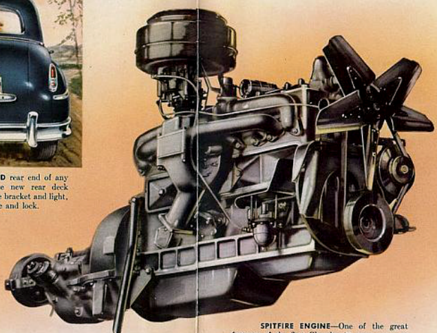
SPITFIRE ENGINE —One of the great features of the first Chrysler 25 years ago was the Chrysler High Compression Engine that revolutionized engine design and performance. In the new Silver Anniversary Models, the Chrysler Spitfire High Compression Engine is the standard by which other power plants will be measured.
